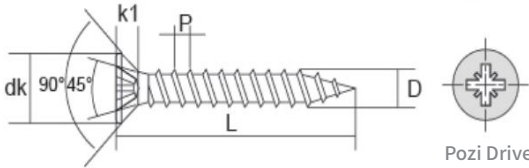
Double flat head Chipboard screw
