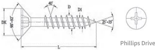
Flat head Chipboard screw
